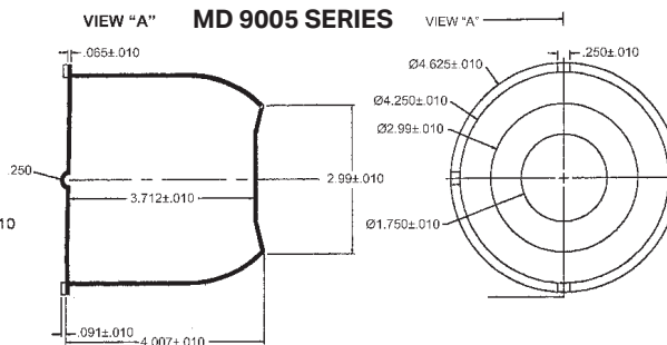
VIEW "A" MD 9005 SERIES
